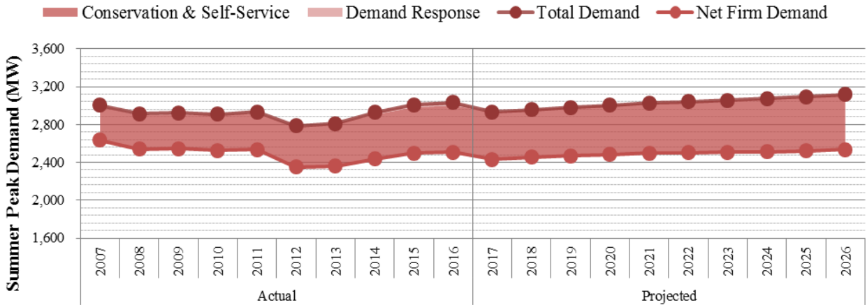
Figure 28: GPC Demand and Energy Forecasts
