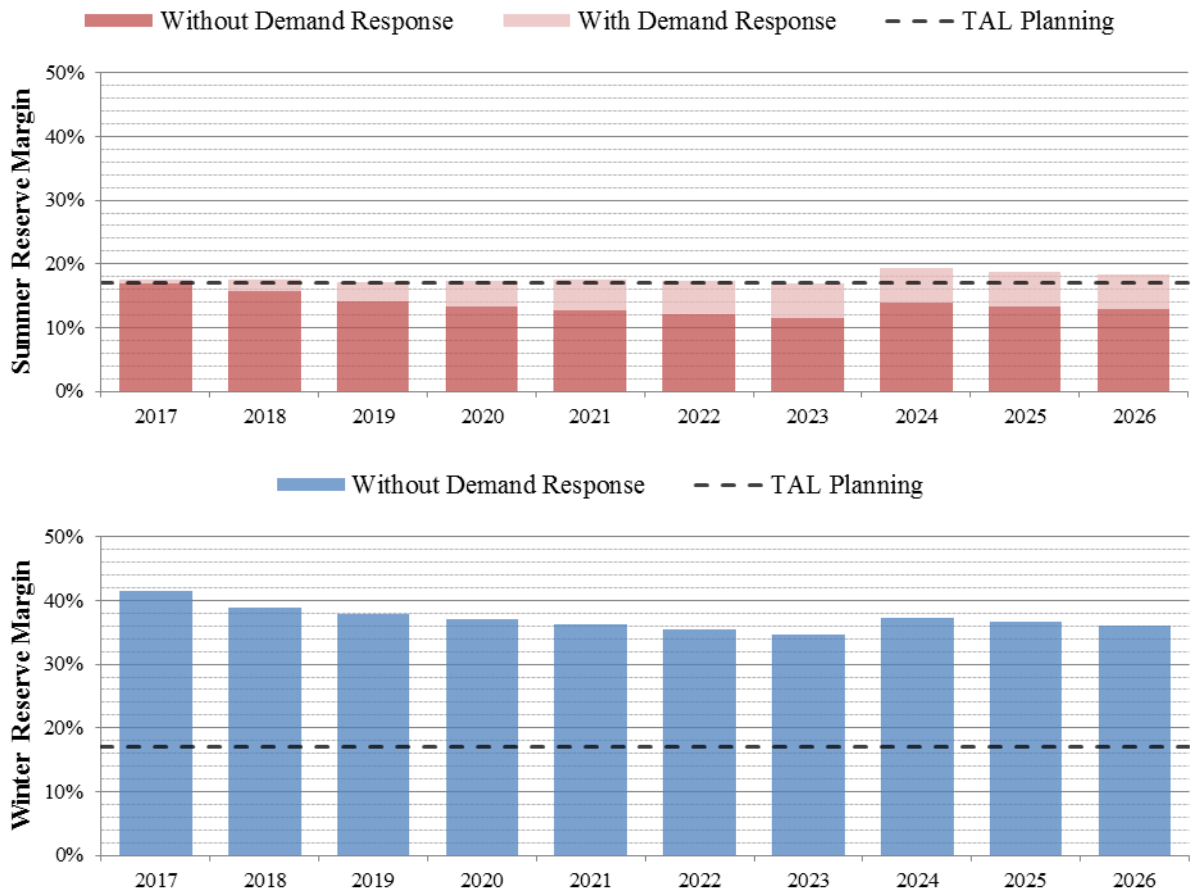
Figure 50: TAL Reserve Margin Forecast
