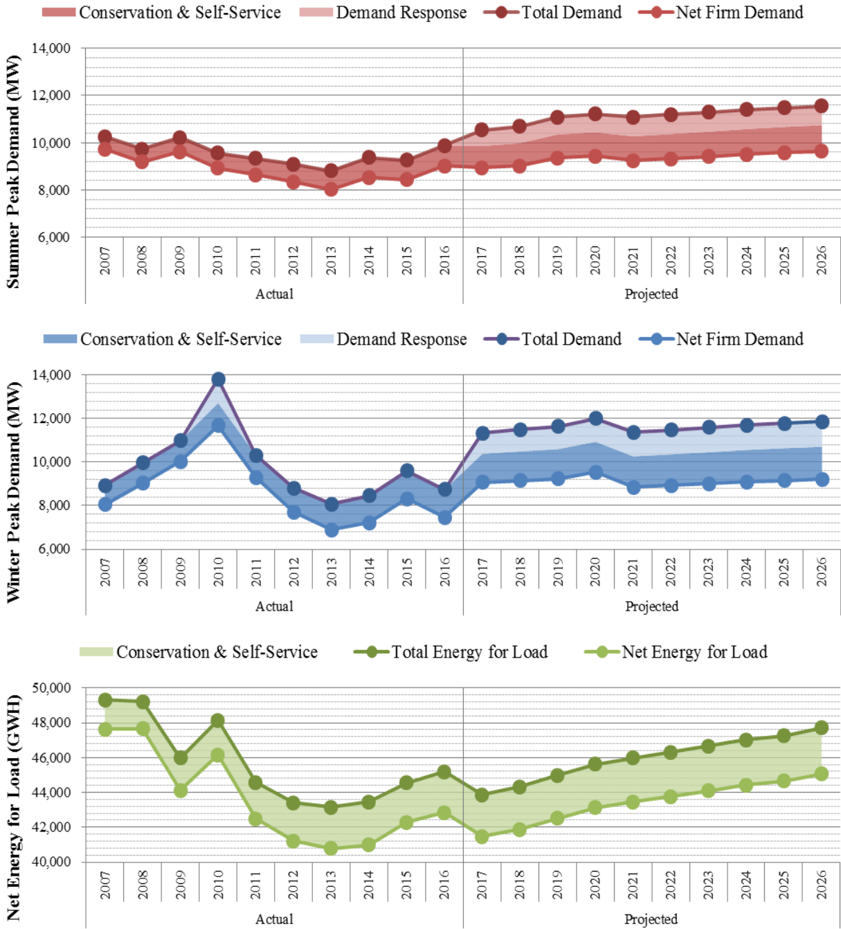
Figure 22: DEF Demand and Energy Forecasts
