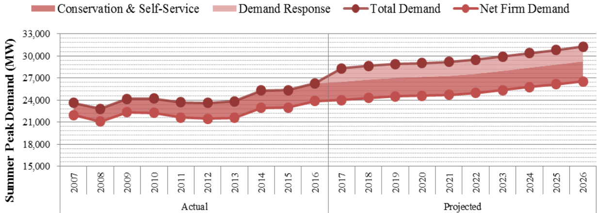
Figure 19: FPL Demand and Energy Forecasts
