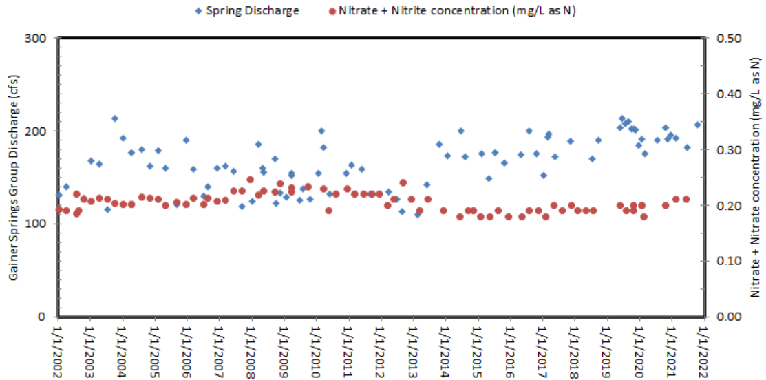
Figure 1.1 Nitrate and Nitrite Concentration and Discharge: Gainer Spring Group (2002-2021)
