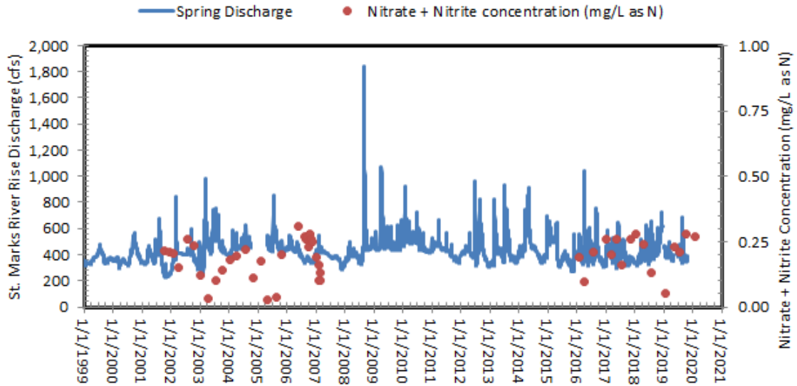
Figure 1.3 Nitrate and Nitrite Concentration and Discharge: St. Marks River Rise (1999-2021)
