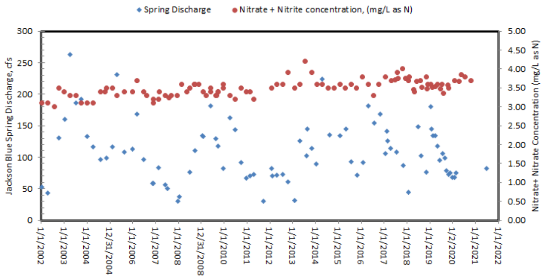
Figure 1.2 Nitrate and Nitrite Concentration and Discharge: Jackson Blue Spring (2002-2021)
