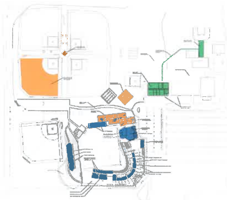
HKS SPORTS & ENTERTAINMENT TIGER TOWN RENOVATIONS LAKELAND, FLORIDA OVERALL SITE PLAN JANUARY 31, 2013
